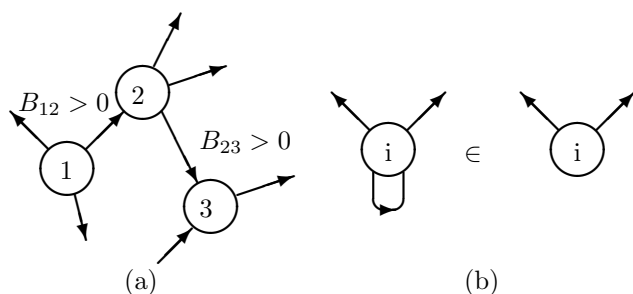
Figure 1: (a) Nodes i and j are considered connected if they have a non-zero B value. Arrows indicate the sign of the B_{ij} value. (b) Self-links are considered internal to a node so B_{ii} = 0 .
