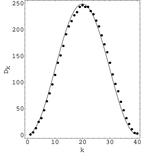
Figure 3: A sample D_k set obtained by numerically maximising \mathcal{P}[D, L, N] where N = 5000 and \log_{10} p = -6 . A curve is also drawn showing that D_k \propto \sin^{d-1}(\pi k/L) , with best fit d = 3.16 and L = 40 .
